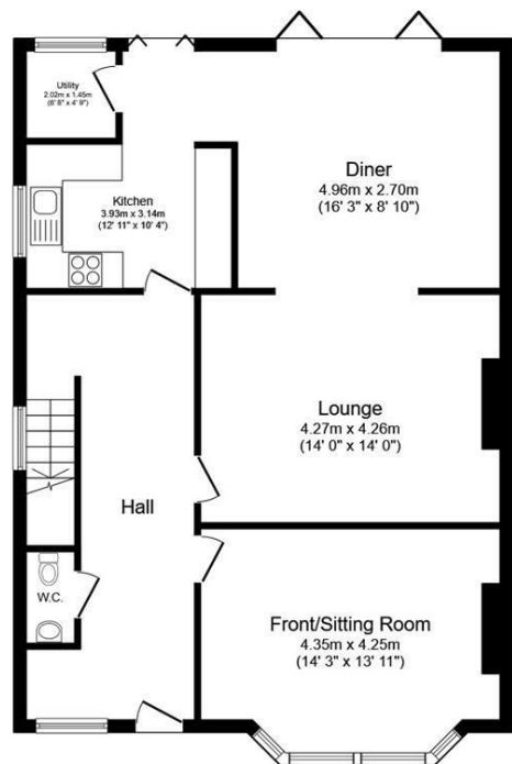
Ground Floor Floor area 88.5 sq.m. (953 sq.ft.)
