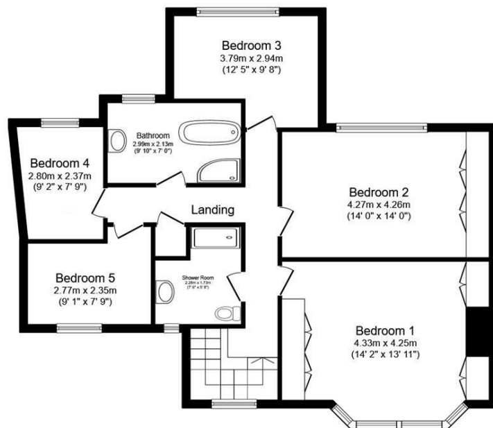
First Floor Floor area 92.0 sq.m. (990 sq.ft.)
